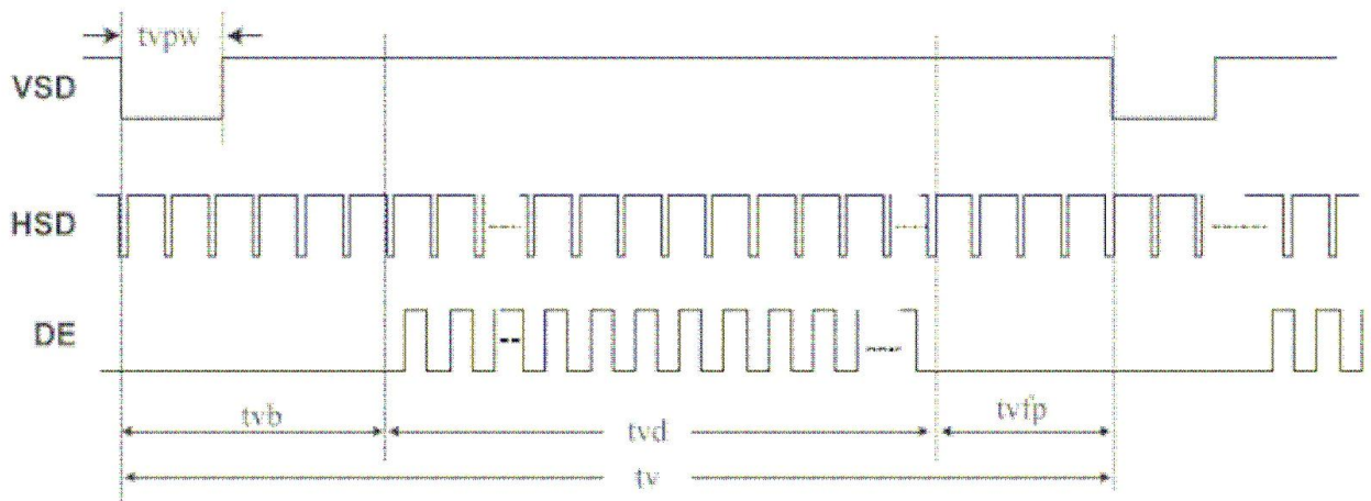
Vertical timing
